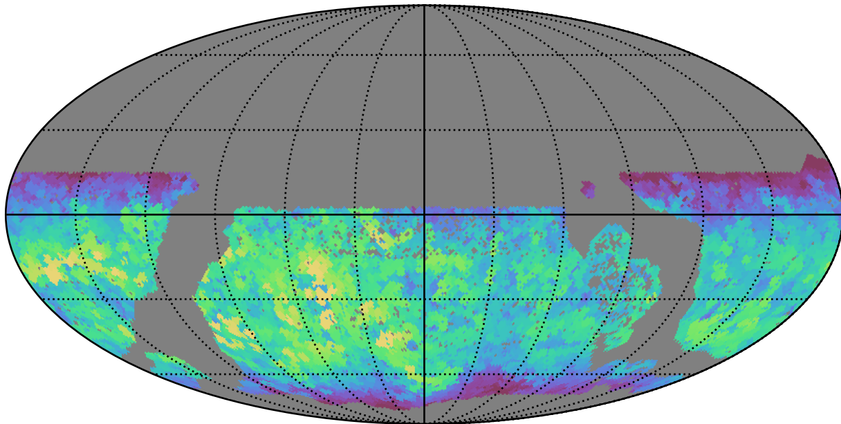
baseline_v3.2_10yrs WFD z band: Max fiveSigmaDepth
