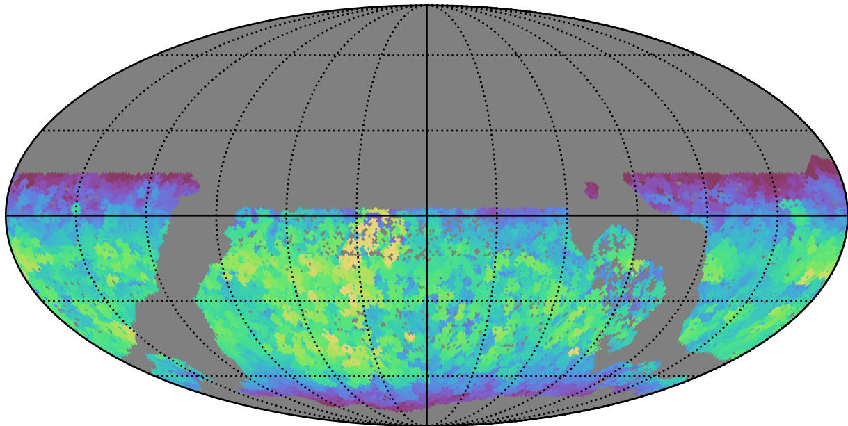
baseline_v3.2_10yrs WFD y band: Max fiveSigmaDepth
