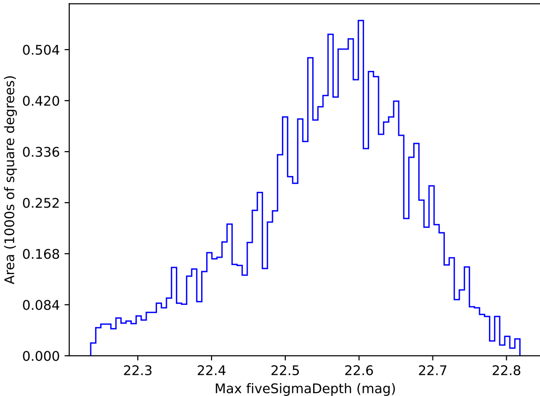
baseline_v3.2_10yrs WFD y band: Max fiveSigmaDepth
