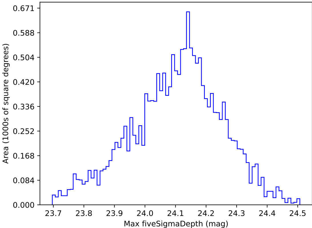
baseline_v3.2_10yrs WFD u band: Max fiveSigmaDepth
