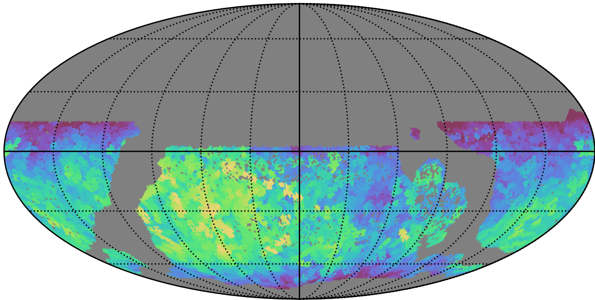
baseline_v3.2_10yrs WFD r band: Max fiveSigmaDepth
