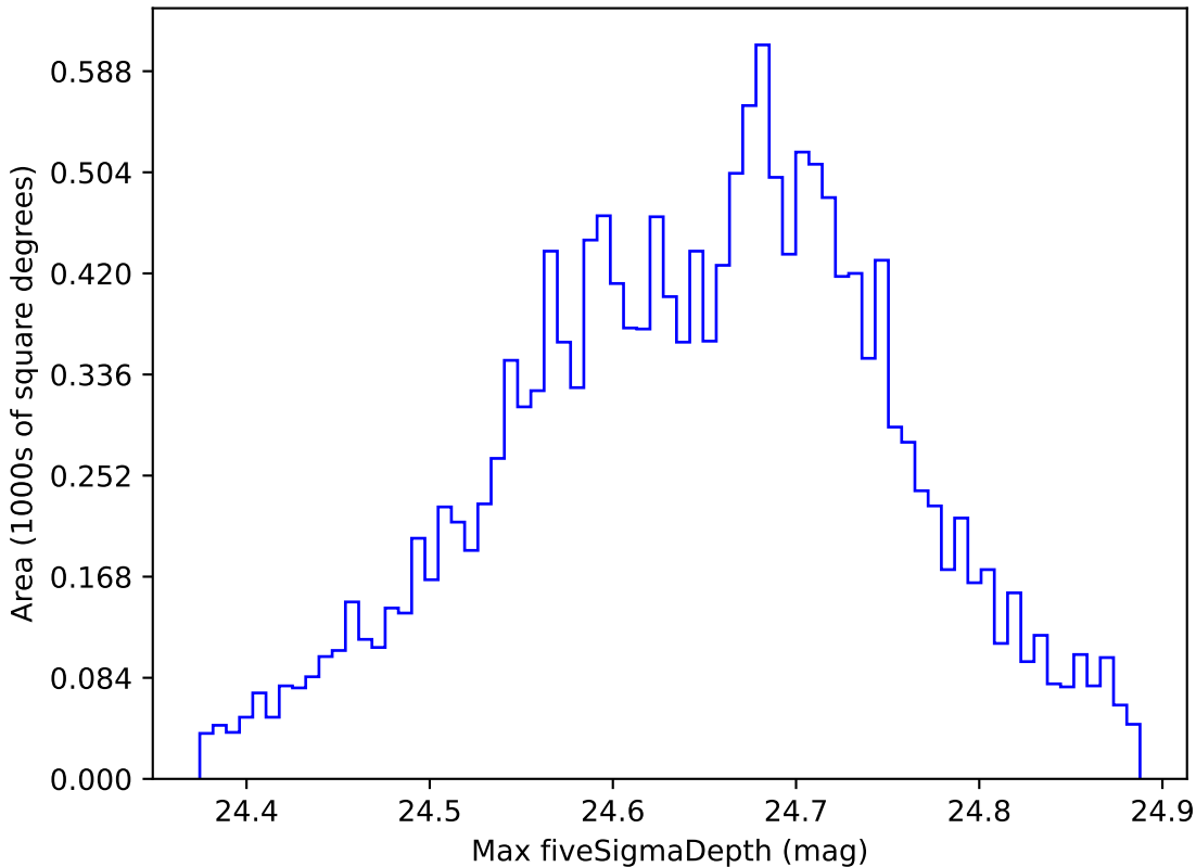
baseline_v3.2_10yrs WFD r band: Max fiveSigmaDepth
