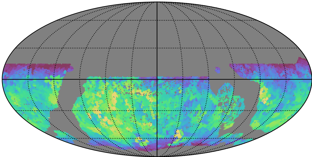
baseline_v3.2_10yrs WFD i band: Max fiveSigmaDepth
