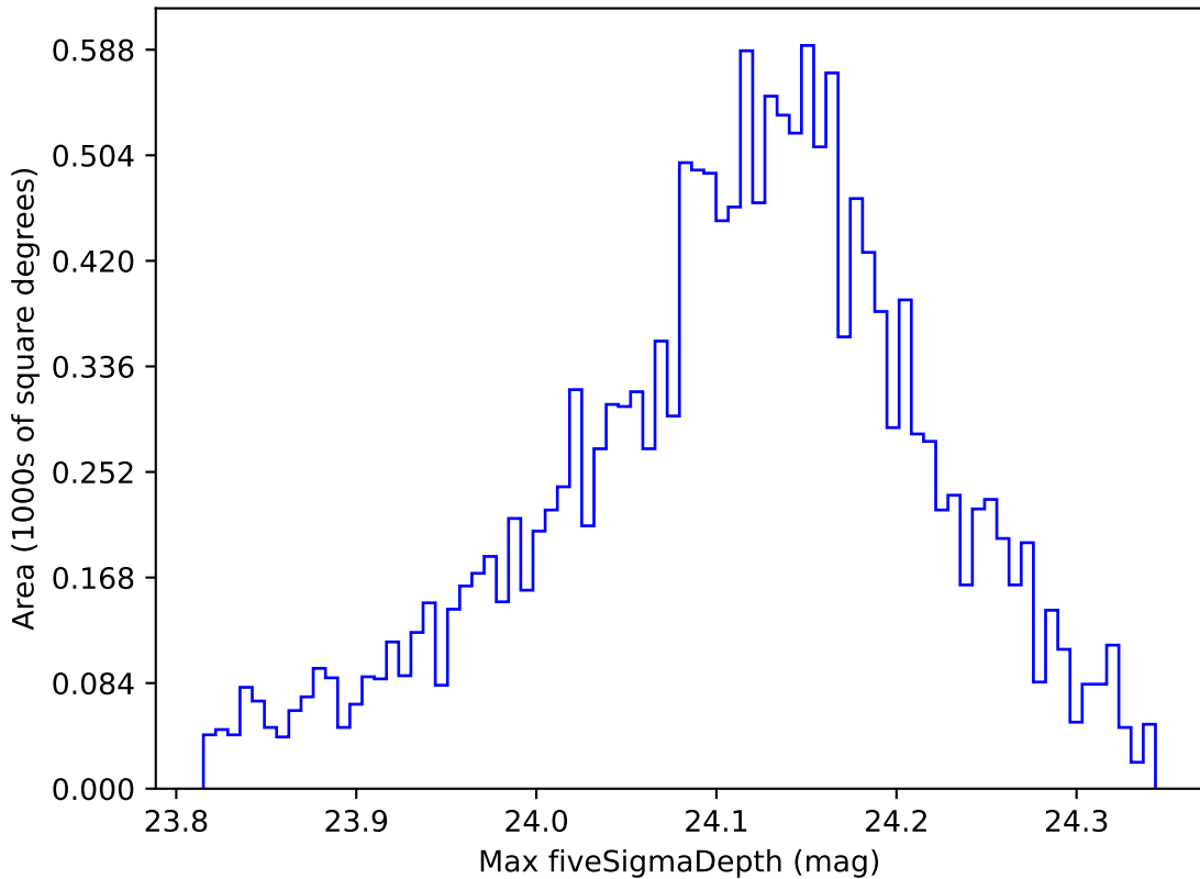
baseline_v3.2_10yrs WFD i band: Max fiveSigmaDepth
