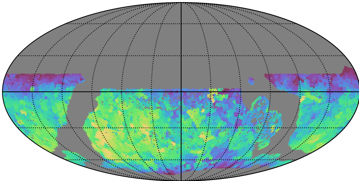
baseline_v3.2_10yrs WFD g band: Max fiveSigmaDepth
