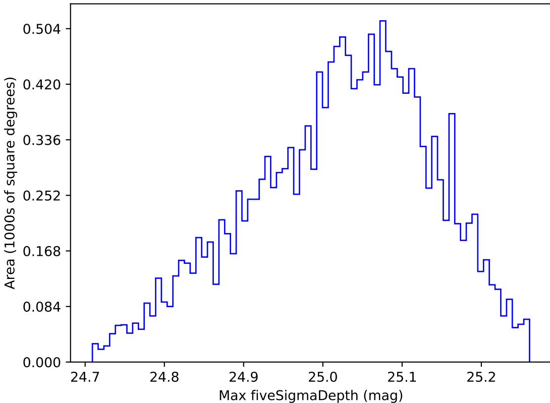
baseline_v3.2_10yrs WFD g band: Max fiveSigmaDepth
