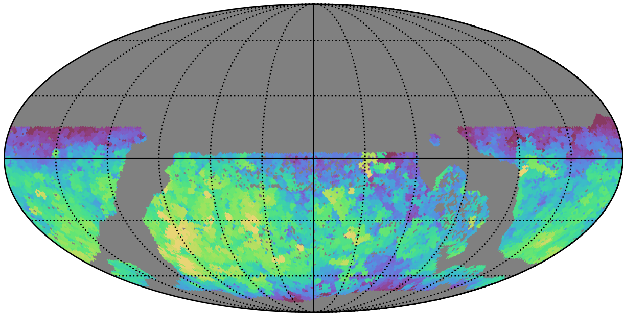
baseline_v3.2_10yrs WFD all bands: Max fiveSigmaDepth
