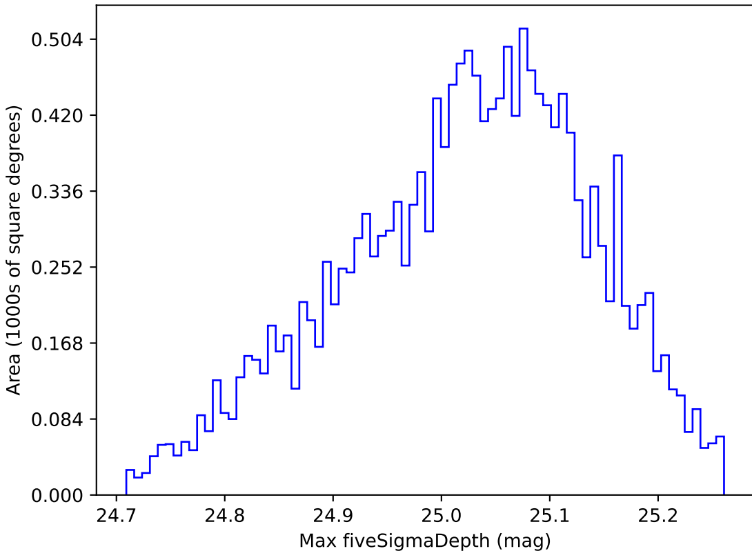
baseline_v3.2_10yrs WFD all bands: Max fiveSigmaDepth
