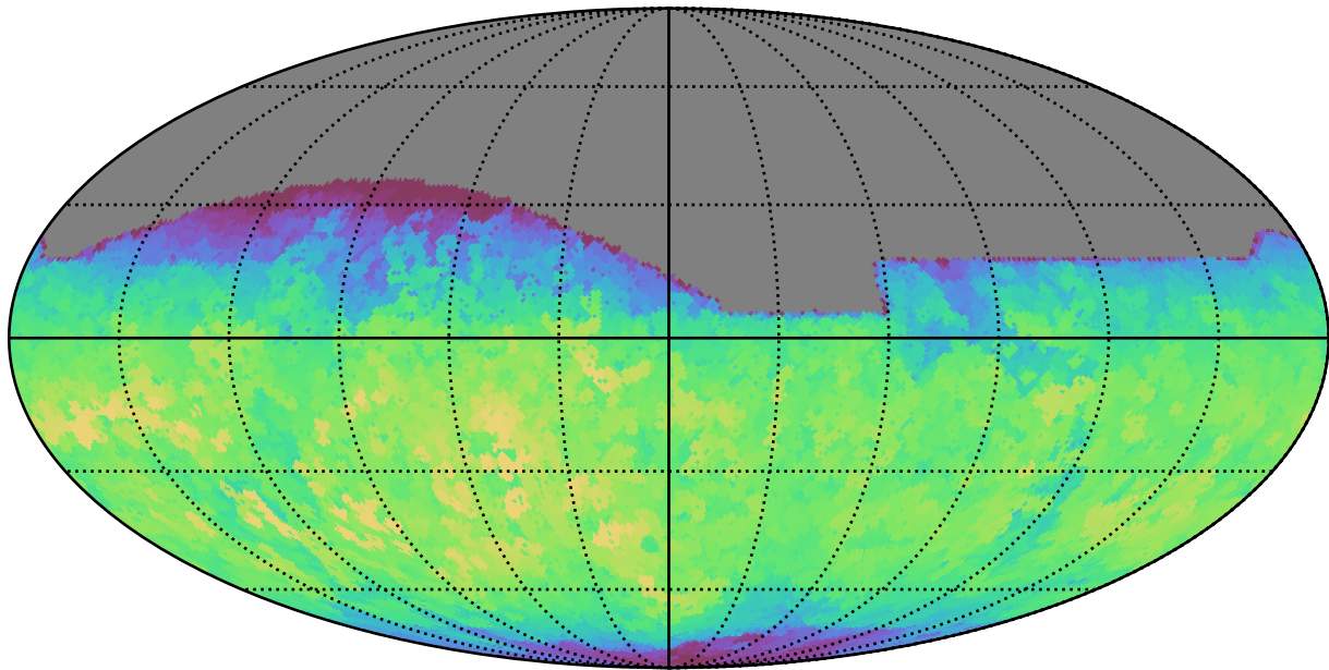
baseline_v3.2_10yrs All sky z band: Max fiveSigmaDepth
