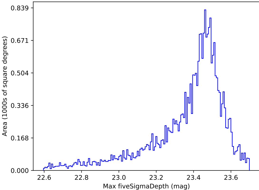
baseline_v3.2_10yrs All sky z band: Max fiveSigmaDepth
