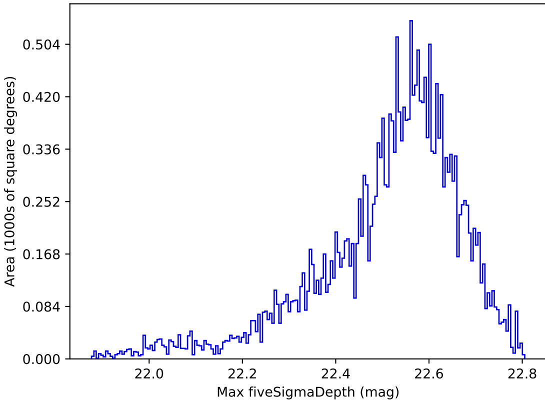
baseline_v3.2_10yrs All sky y band: Max fiveSigmaDepth
