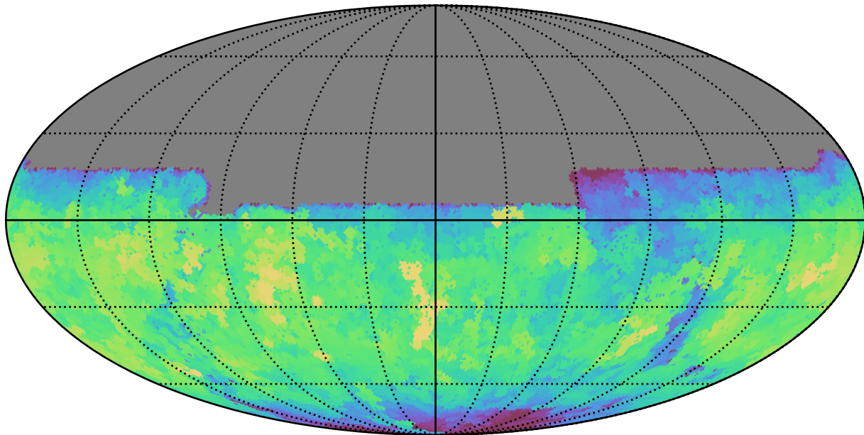
baseline_v3.2_10yrs All sky u band: Max fiveSigmaDepth
