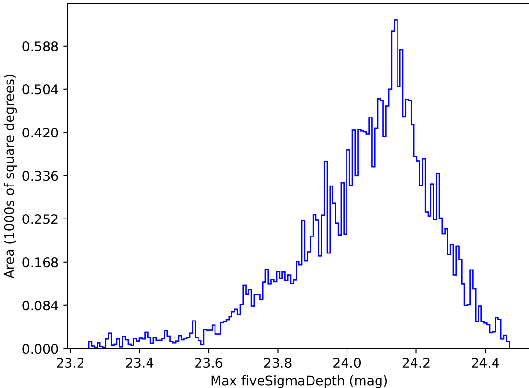
baseline_v3.2_10yrs All sky u band: Max fiveSigmaDepth
