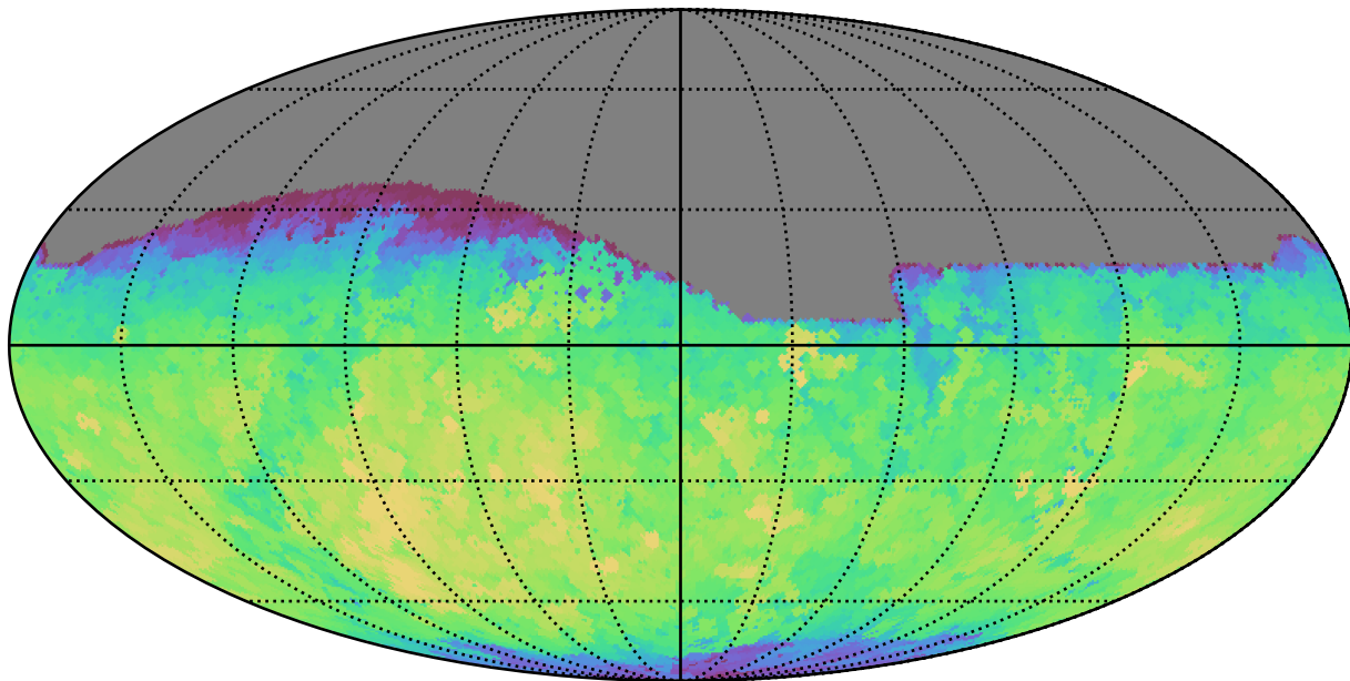
baseline_v3.2_10yrs All sky g band: Max fiveSigmaDepth
