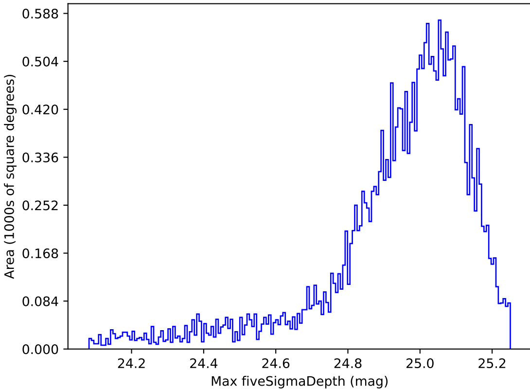
baseline_v3.2_10yrs All sky g band: Max fiveSigmaDepth
