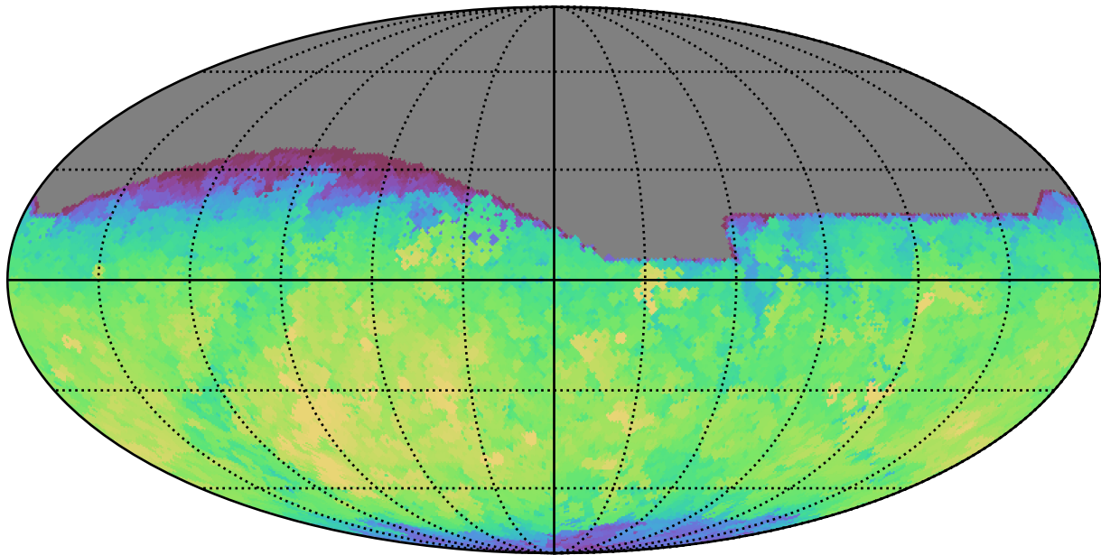
baseline_v3.2_10yrs All sky all bands: Max fiveSigmaDepth
