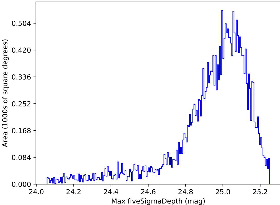
baseline_v3.2_10yrs All sky all bands: Max fiveSigmaDepth
