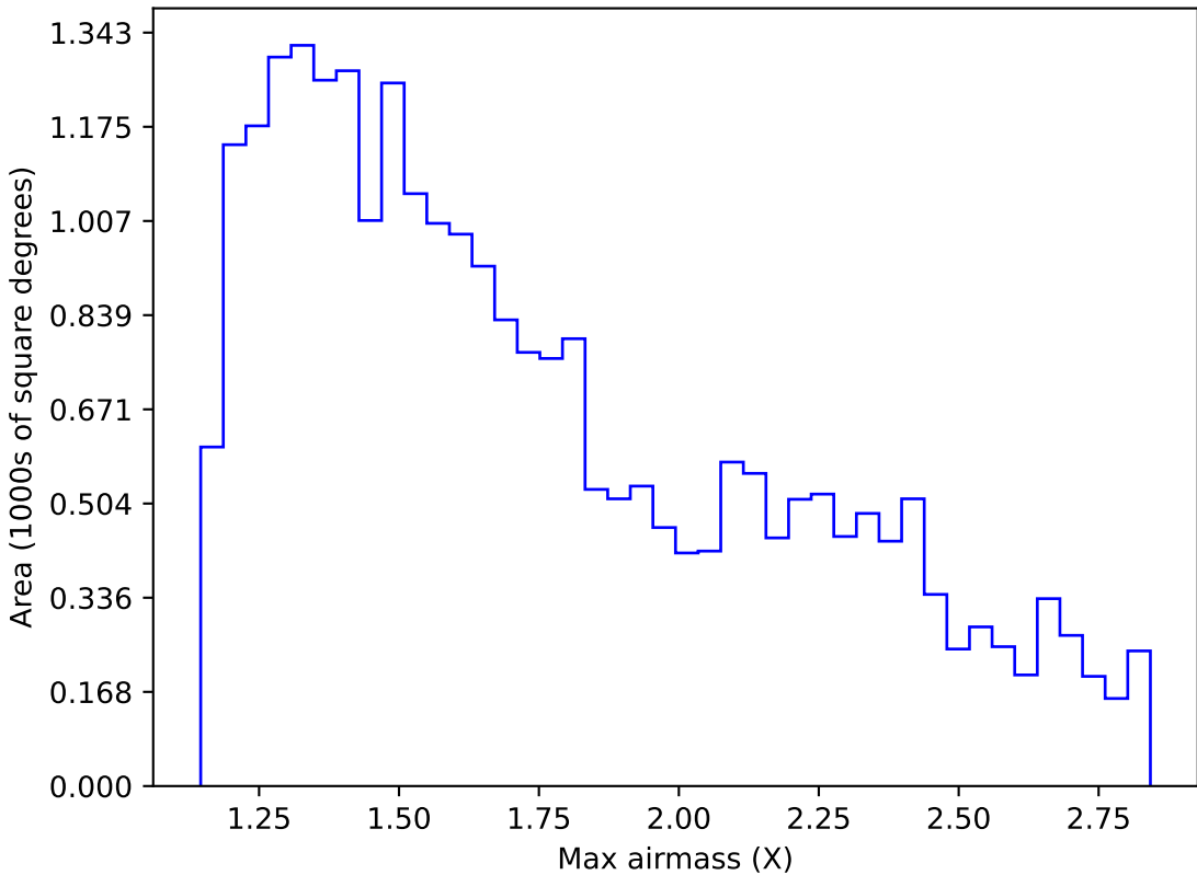
baseline_v3.2_10yrs Yr 1 z band: Max airmass
