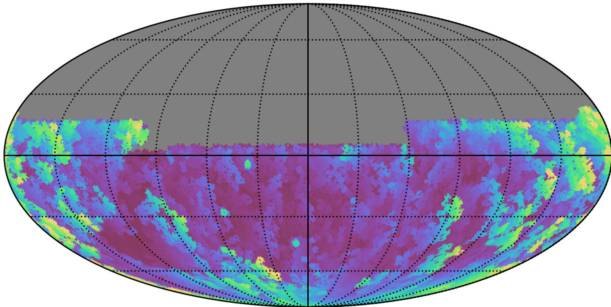
baseline_v3.2_10yrs Yr 1 y band: Max airmass
