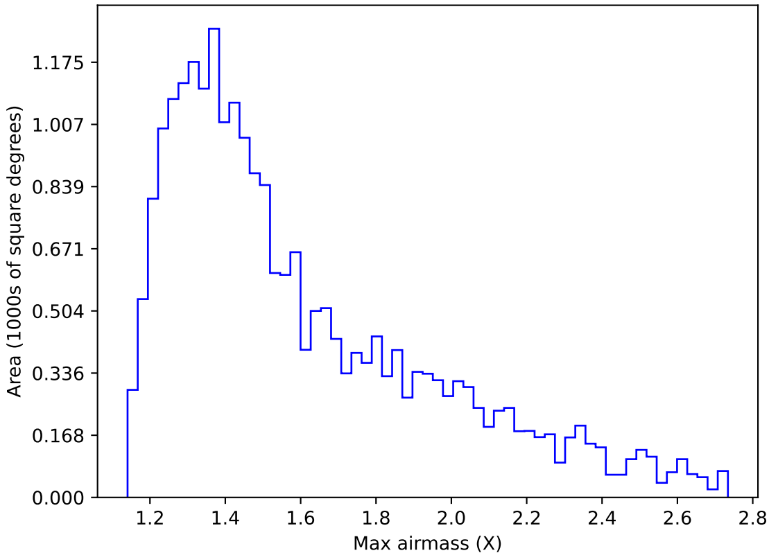
baseline_v3.2_10yrs Yr 1 y band: Max airmass
