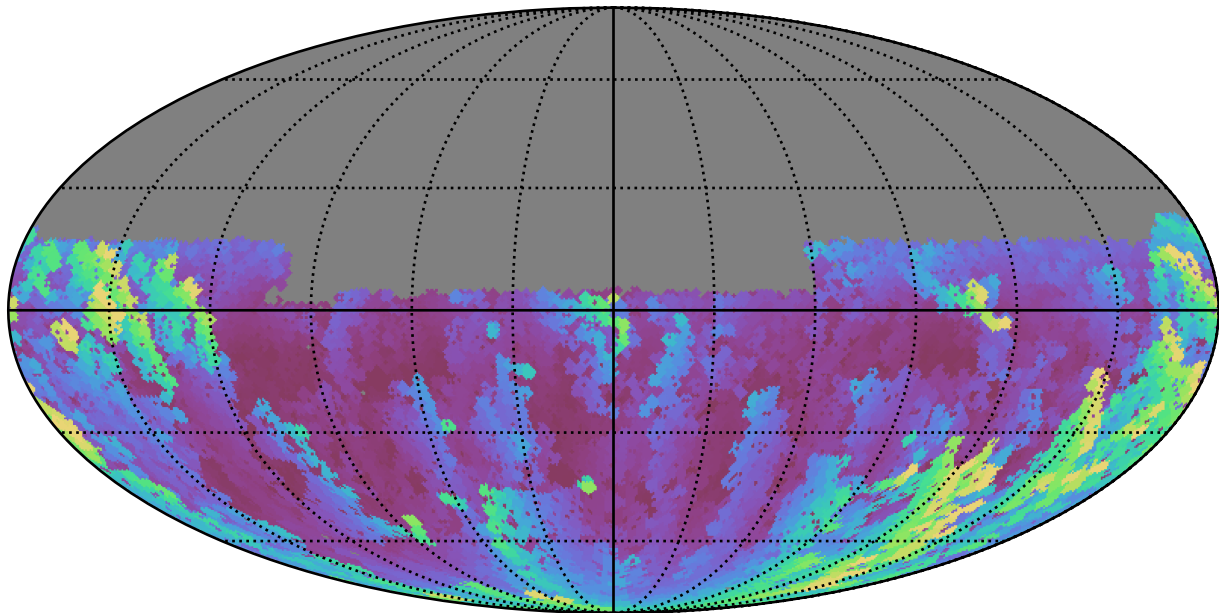
baseline_v3.2_10yrs Yr 1 u band: Max airmass
