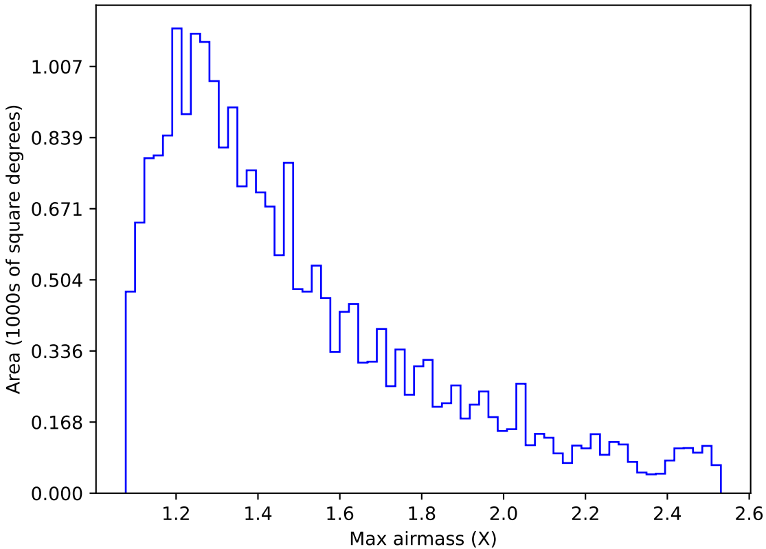
baseline_v3.2_10yrs Yr 1 u band: Max airmass
