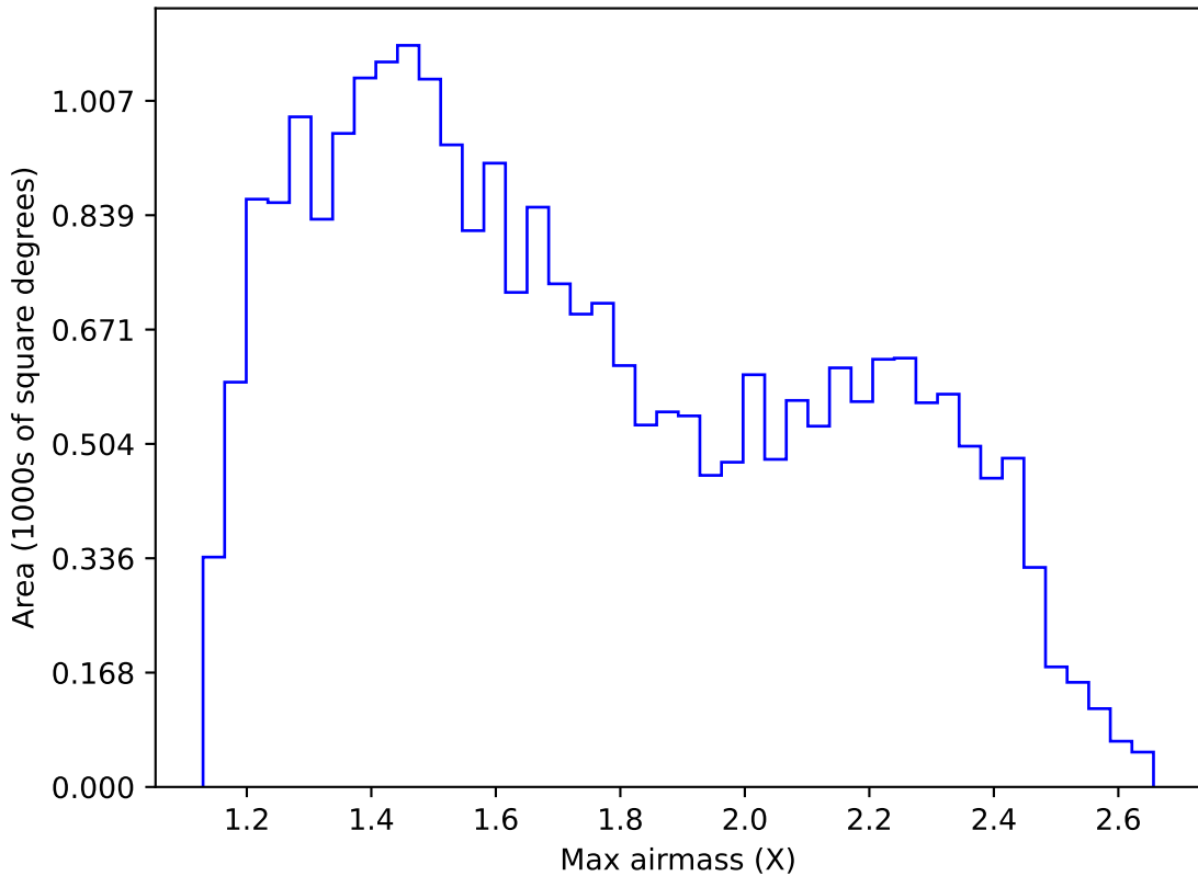
baseline_v3.2_10yrs Yr 1 r band: Max airmass
