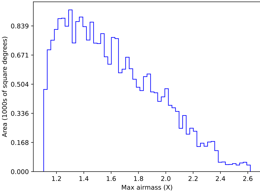
baseline_v3.2_10yrs Yr 1 g band: Max airmass
