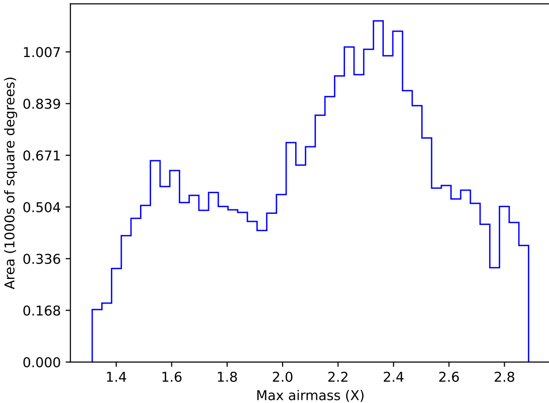
baseline_v3.2_10yrs Yr 1 all bands: Max airmass
