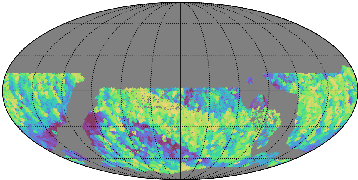
baseline_v3.2_10yrs WFD z band: Max airmass
