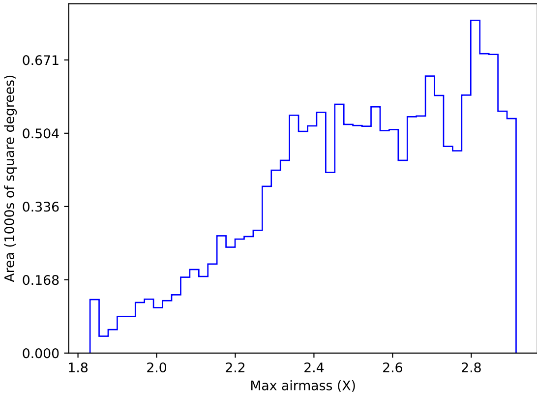
baseline_v3.2_10yrs WFD z band: Max airmass
