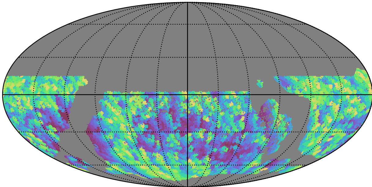
baseline_v3.2_10yrs WFD y band: Max airmass
