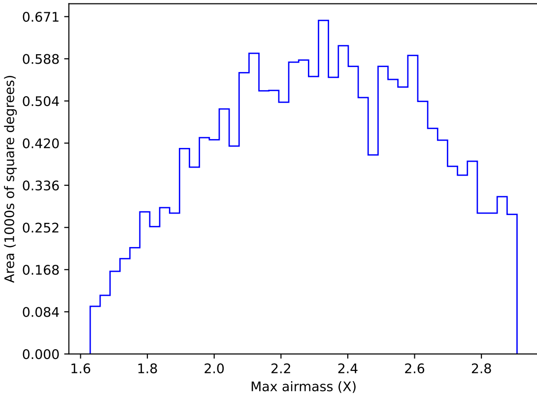
baseline_v3.2_10yrs WFD y band: Max airmass
