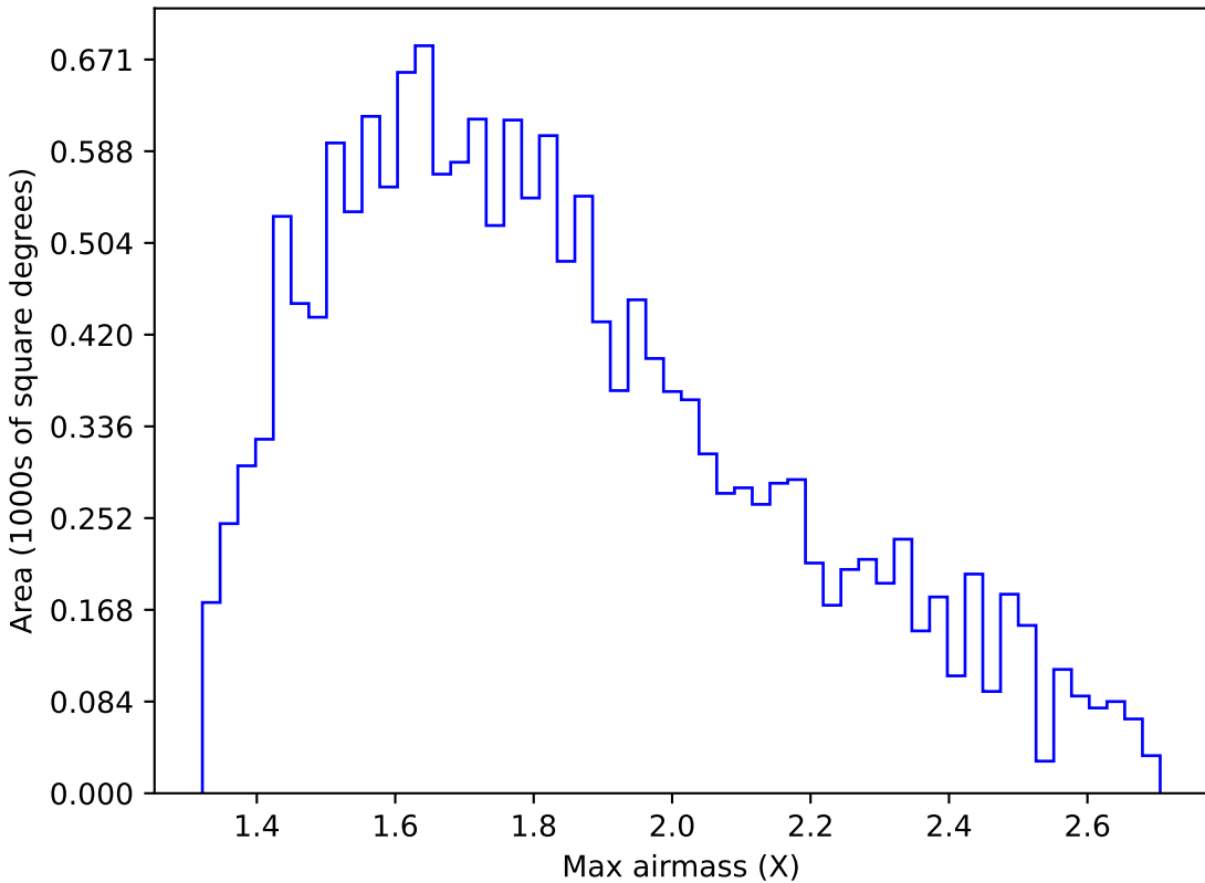
baseline_v3.2_10yrs WFD u band: Max airmass
