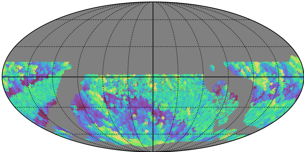
baseline_v3.2_10yrs WFD r band: Max airmass
