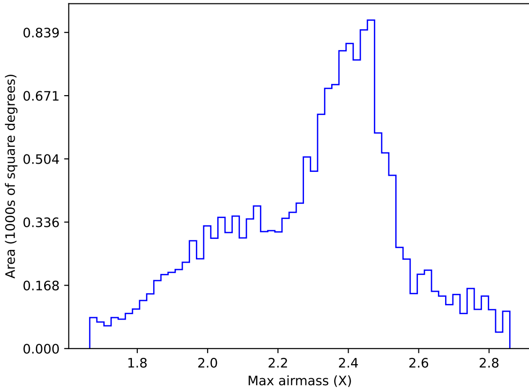
baseline_v3.2_10yrs WFD r band: Max airmass
