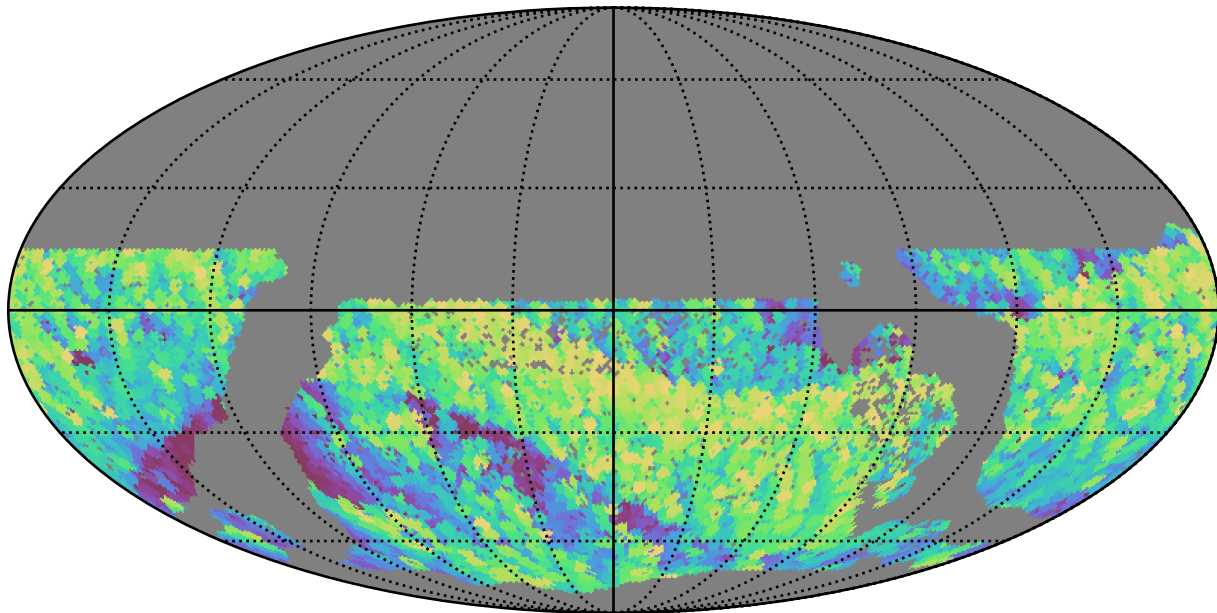
baseline_v3.2_10yrs WFD i band: Max airmass
