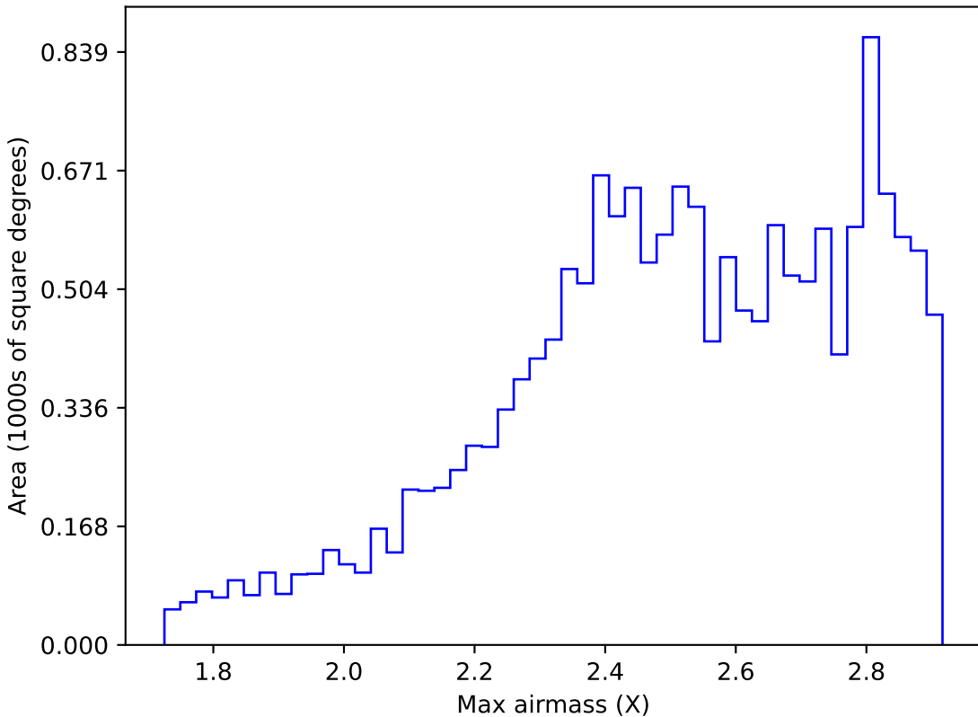
baseline_v3.2_10yrs WFD i band: Max airmass
