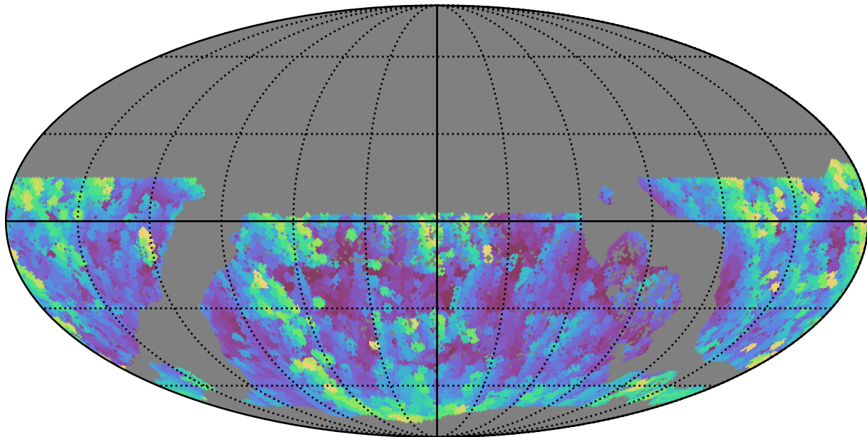
baseline_v3.2_10yrs WFD g band: Max airmass
