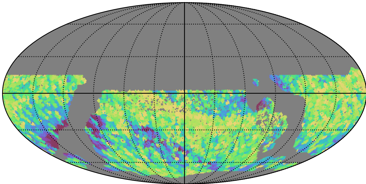
baseline_v3.2_10yrs WFD all bands: Max airmass
