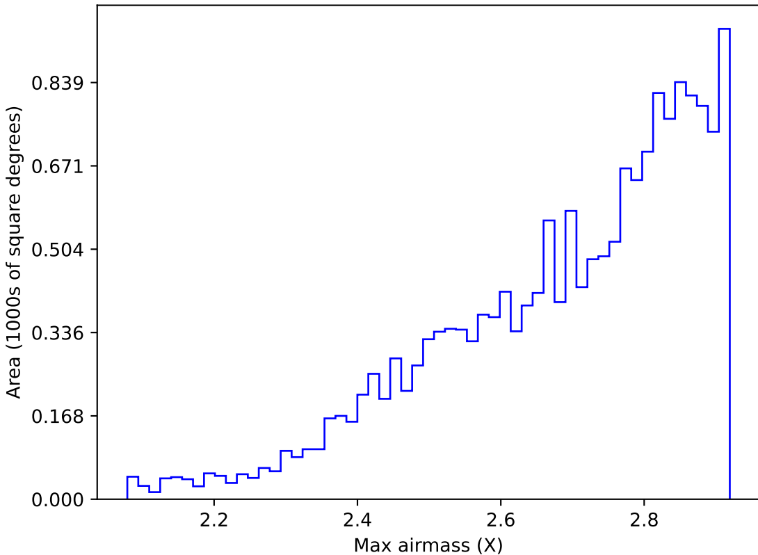
baseline_v3.2_10yrs WFD all bands: Max airmass
