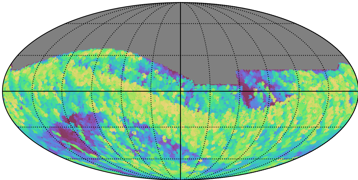
baseline_v3.2_10yrs All sky z band: Max airmass
