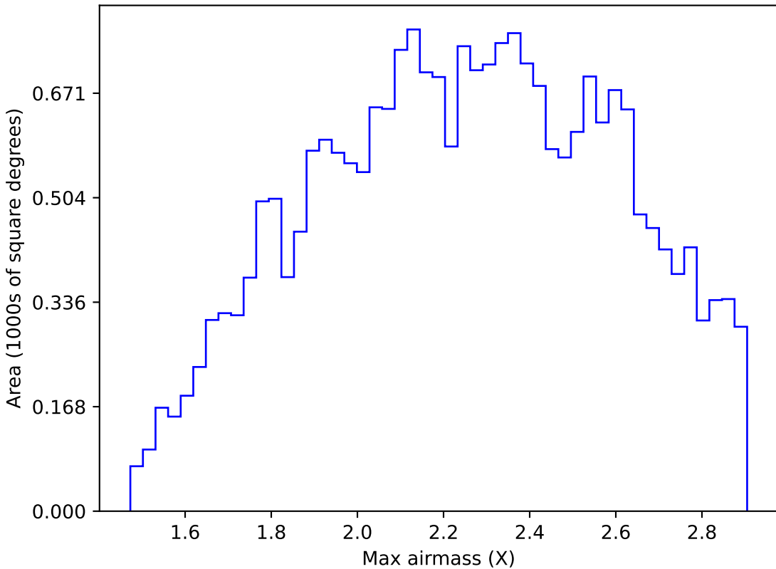
baseline_v3.2_10yrs All sky y band: Max airmass
