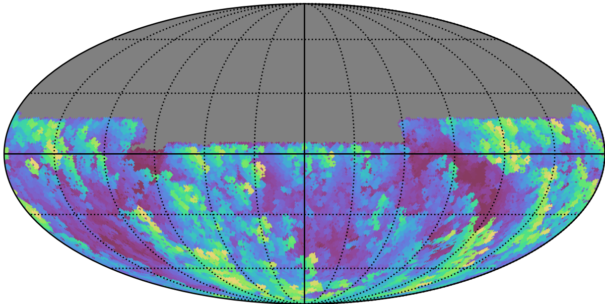
baseline_v3.2_10yrs All sky u band: Max airmass
