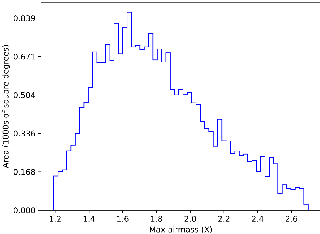
baseline_v3.2_10yrs All sky u band: Max airmass
