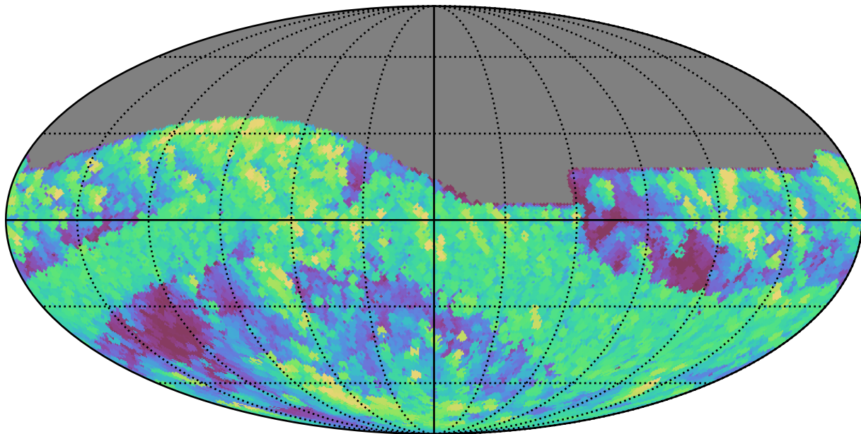
baseline_v3.2_10yrs All sky r band: Max airmass
