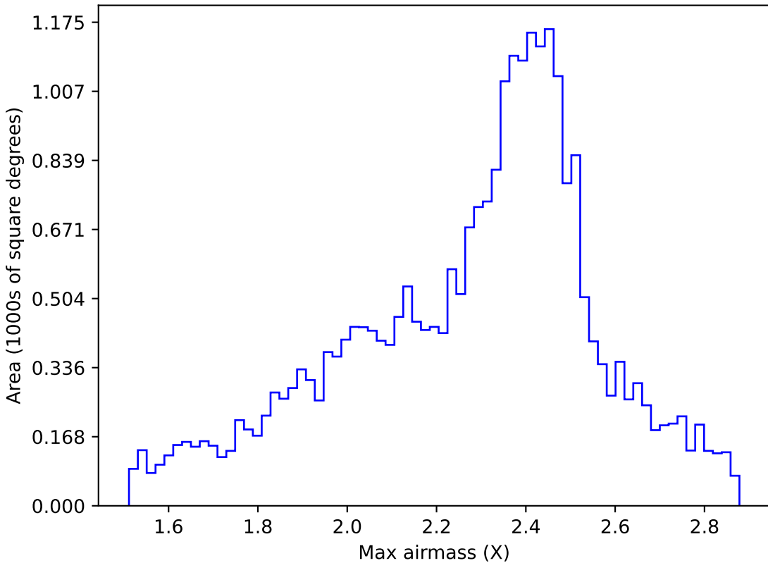
baseline_v3.2_10yrs All sky r band: Max airmass
