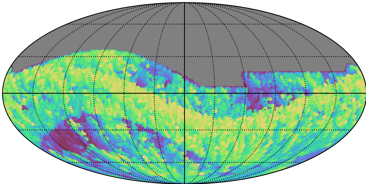
baseline_v3.2_10yrs All sky i band: Max airmass
