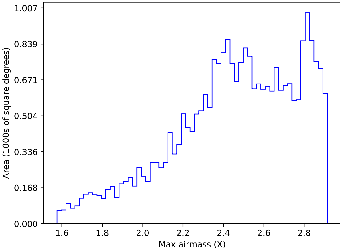
baseline_v3.2_10yrs All sky i band: Max airmass
