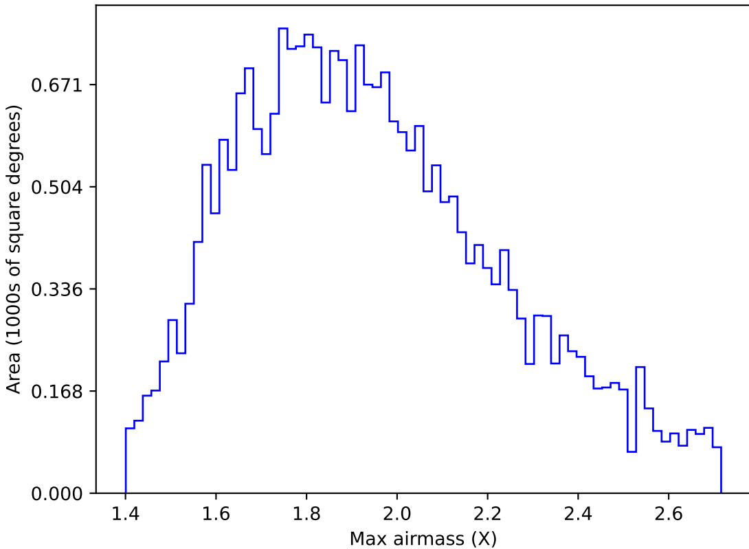
baseline_v3.2_10yrs All sky g band: Max airmass
